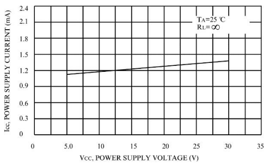
Figure 5. Power Supply Current versus Power Supply Voltage
